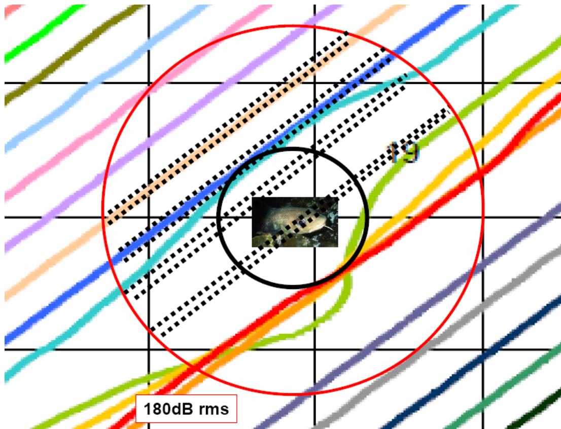
Figure 3. View from above. Simple modelling of deleterious noise around a marine fish when staying in a fixed position at the seabed with a seismic vessel passing above along transect lines. Each black dot is one firing of the airgun array. The red circle (the "danger zone") is 3 km in diameter.
