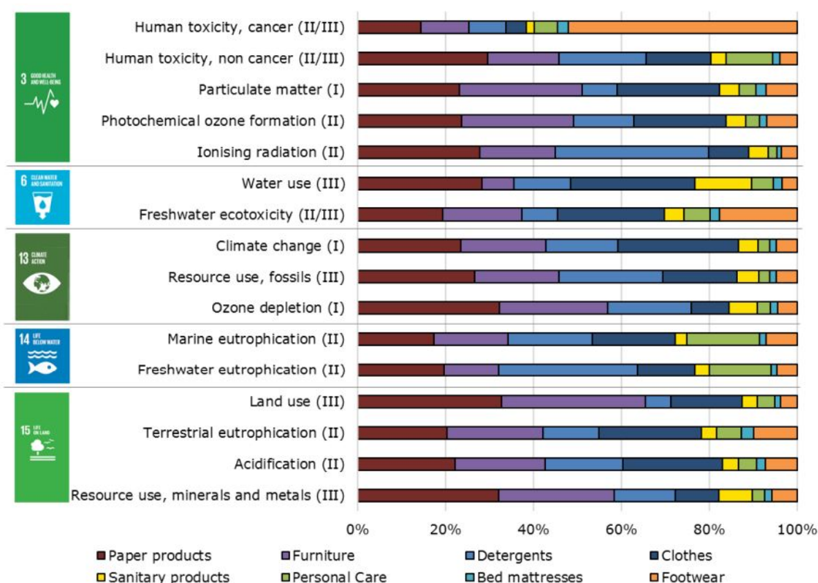
Figure R2.9: Contribution of different products to the impacts of household goods in EU in 2010. The roman numbers in brackets reffer to the robustness of the model used to assess environmental impacts. The lower the number, the higher its robustness. Figure from Beylot et al. (2019).
