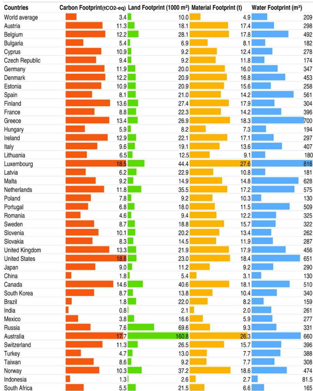
Figure R2.7: Environmental footprints of household consumption across countries for year 2007. The figure includes the world average and 43 selected countries from EXIOBASE 2.2, ordered alphabetically by country codes. The world average includes all 43 countries and the five rest-of-the-world regions. Figure from Ivanova et al. (2016).
