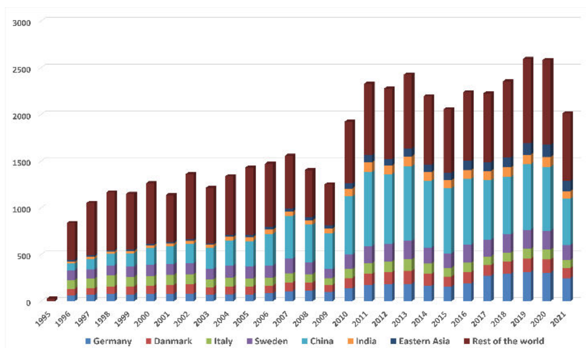
Figure R2.11: Norwegian direct imports of clothing articles from EXIOBASE 3.8.2 with a breakdown on the top supplying countries and regions for 1995 – 2021 in million Euro.
